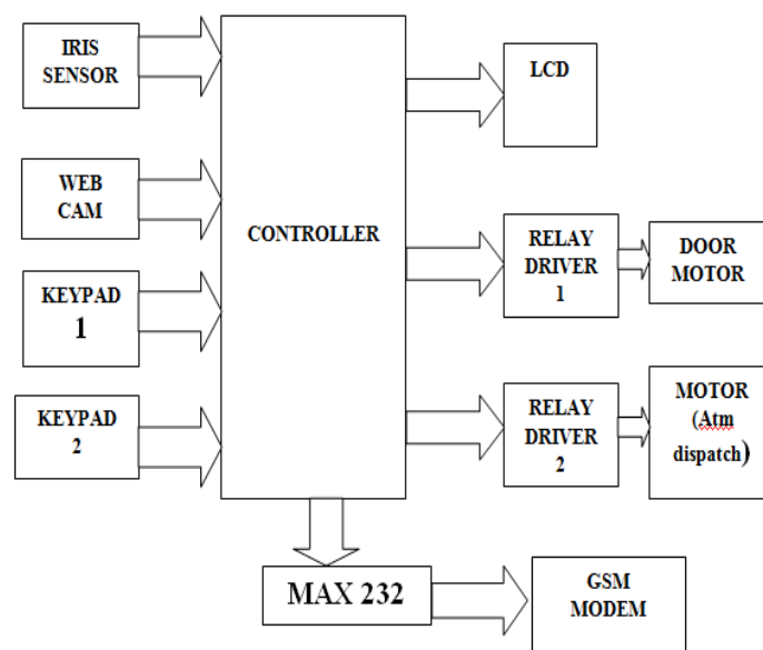
Fig 2: BLOCK DIAGRAM OF ATM USING RASPBERRY PI
